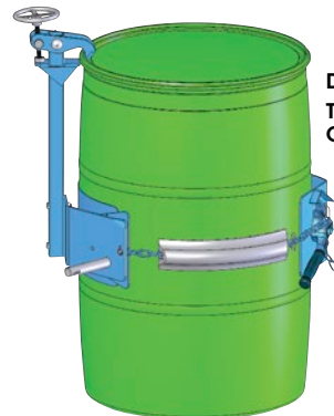
DC279 Bracket Assembly
